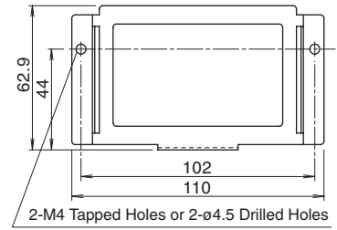
PS9Z-5R2B Panel Mounting Bracket
