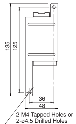
PS9Z-5R1E Panel Mounting Bracket
