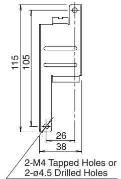
PS9Z-5R1C Panel Mounting Bracket
